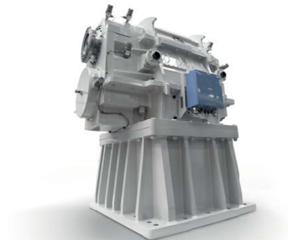
RSB 660: 54 MW gas turbine load gearbox
