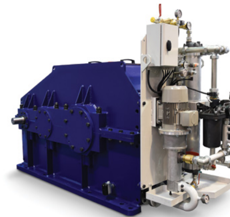
High-speed gearbox for steam turbine-driven cane mill
