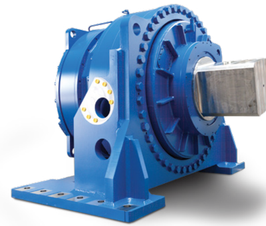
Coaxial 1,500 HP OrbifleX® gearbox for cane mill drive
