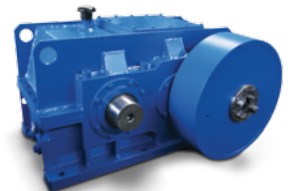
Helical gearbox for cutting shears
