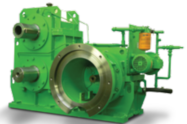
Two-roll calender gearbox
