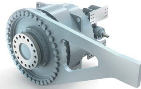
Bevel-planetary gearbox Orbi-flex for track drive
