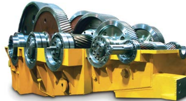
Gearbox for jib elevation and extension of KU 800 excavator
