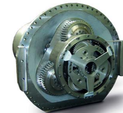
Planetary haul truck axle gearbox
