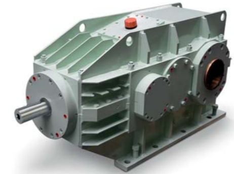
Belt conveyor drive gearbox
