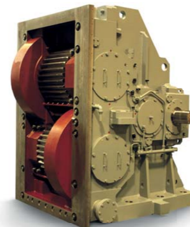
Horizontal ball mill gearbox of SD type (4.1 - 6.0 MW)
