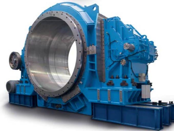
Two SD 2.0 MW gearboxes with integrated girth gear
